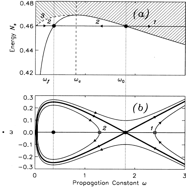
FIG. 3. (a) Characteristic dependence of the soliton energy N_s(\omega) for \sigma = -1 and 2 < p < 4 (here we select p = 3.3 ). The points \omega_f , \omega_c , and \omega_0 have the same meaning as in Fig. 2(a). Shaded region determines the soliton collapse, while the region 2 corresponds to the periodic amplitude oscillations. (b) Phase plane (\omega, \dot{\omega}) of the analytical model (13) describing different regimes of the soliton dynamics: curve 1—soliton collapse; curve 2—amplitude oscillations around the stable solution with \omega = \omega_f .
